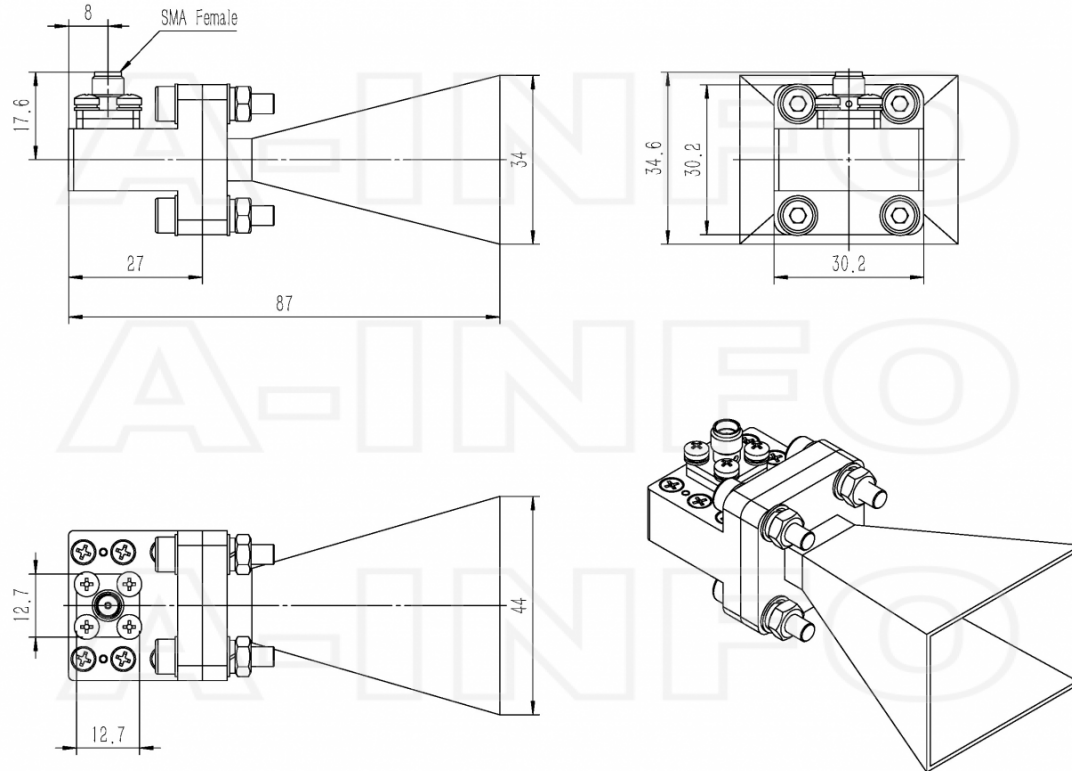
SMA-Female Output (P/N: LB-51-15-C-SF)
